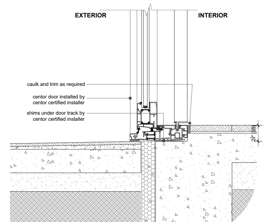
typical rough opening clearances
