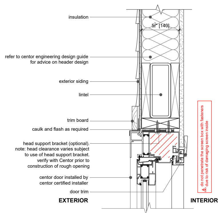
2b head detail section
