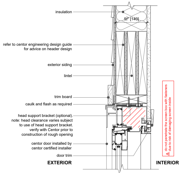
2a head detail section
